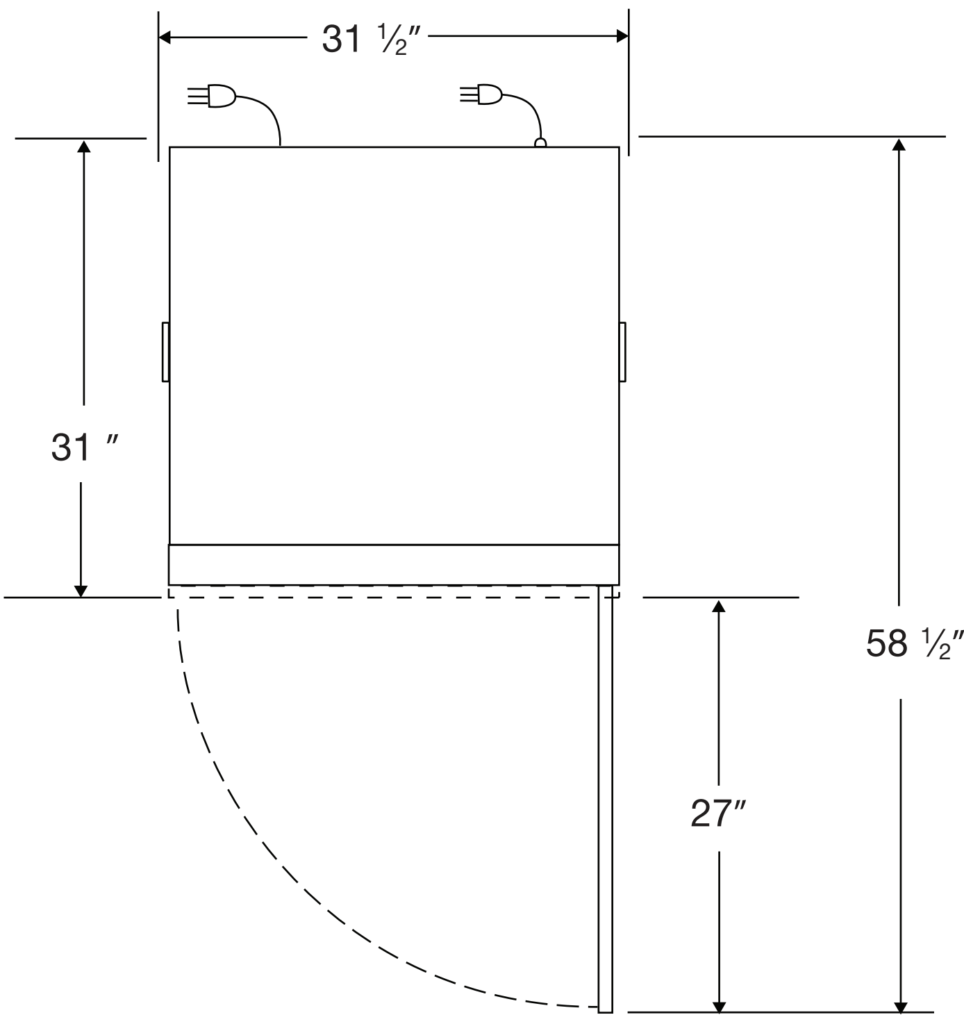
Top View
