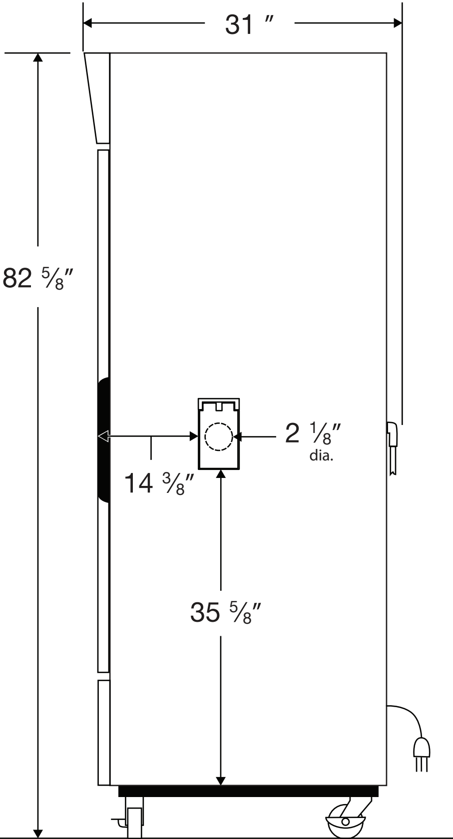
Side View
