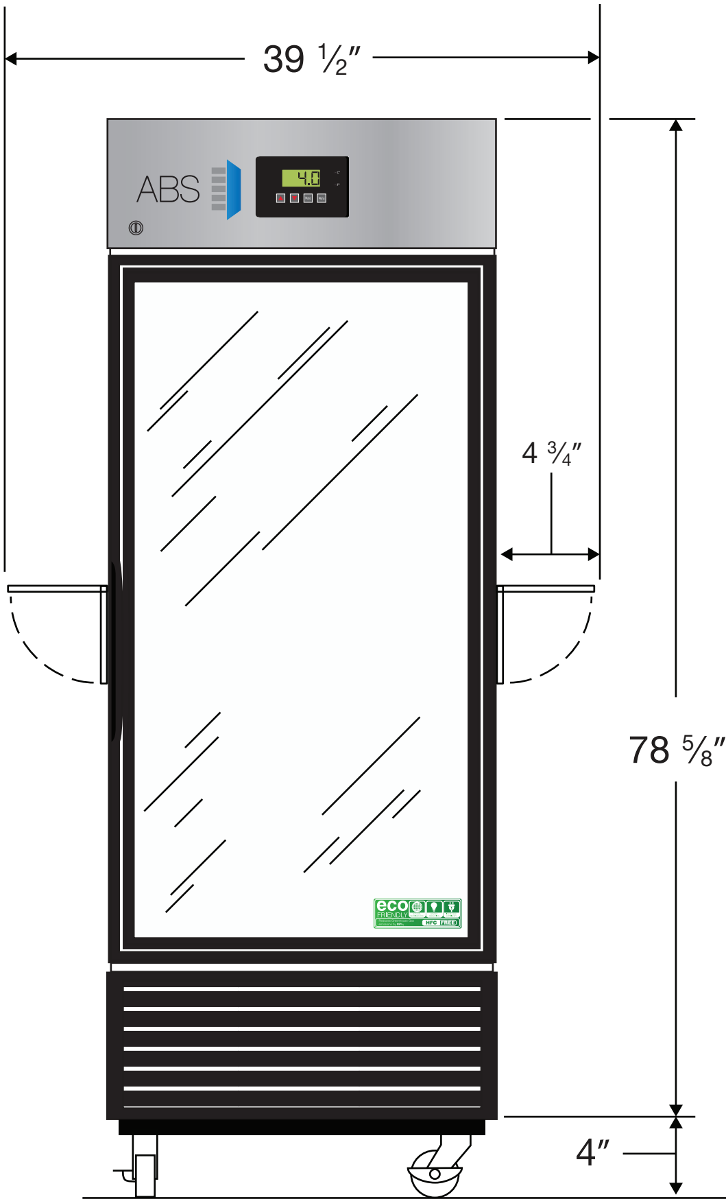
Front View
