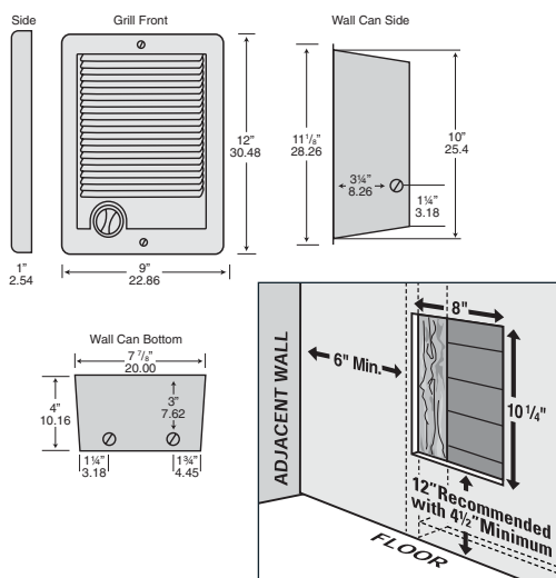
ROUGH-IN: 8" W x 10-1/8" H x 4" D
