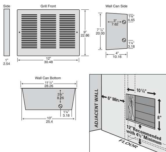
ROUGH-IN: 10-1/8" W x 8" H x 4" D
