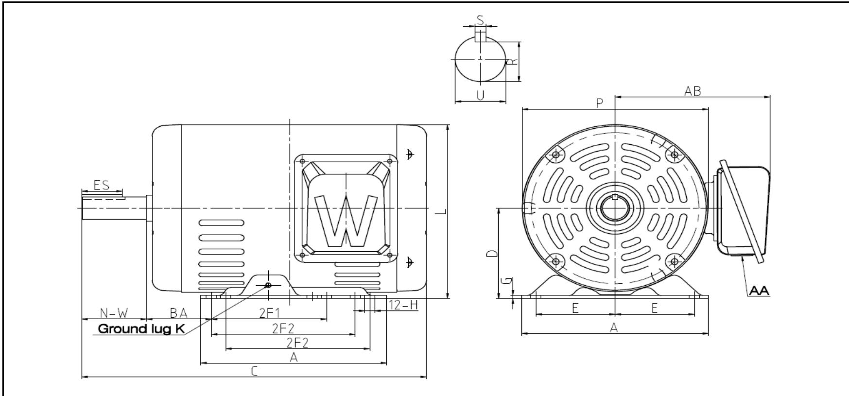
DIMENSIONS - INCHES
