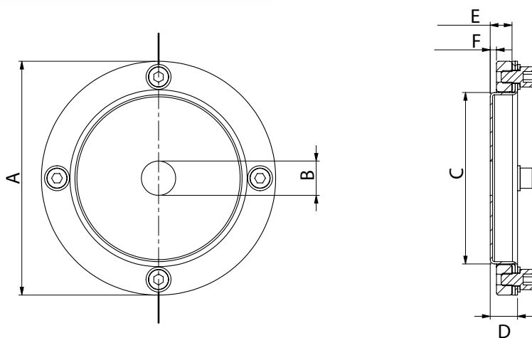
DIMENSIONAL SPECIFICATIONS
