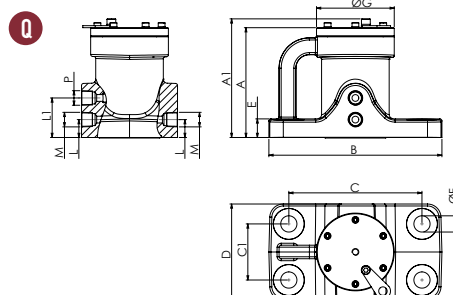
DIMENSIONAL SPECIFICATIONS
