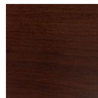
Mahogany (MH)
