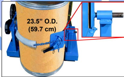
...to your 23.5" (59.7 cm) diameter drum... ...and any size in between
