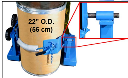
The MORCINCH™ drum holder automatically adjusts from your 22" (56 cm) diameter drum...
