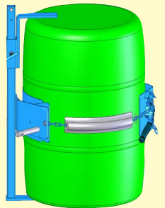
Kit # 4556-P shown bolted onto MORCINCH™ drum holder
