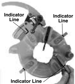
Figure 12 – Inserting Dies
