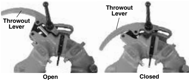
Figure 11 – Open/Closed Position
