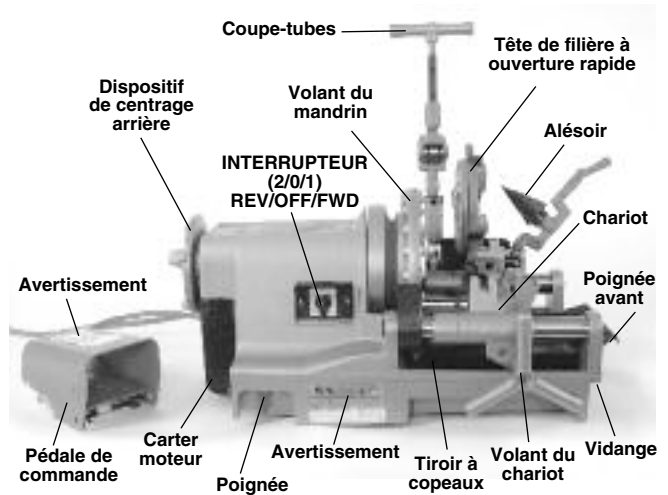
Figure 1 – Fileteuse 300 Compact
