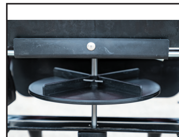
Large 9 in. spinner spreads up to 24 ft.
