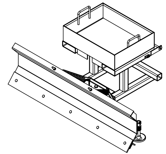
ISOMETRIC VIEW SHOWS WEIGHT BOX ON TOP OF SPB-N-72 SNOW PLOW
