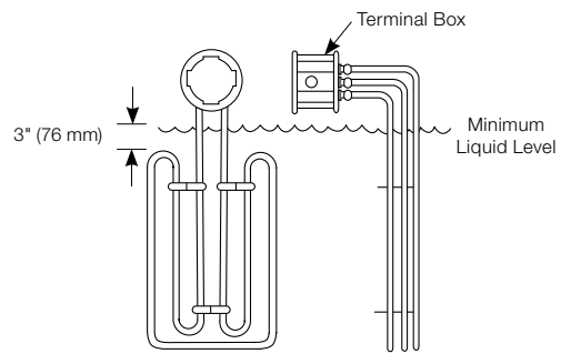
Over-the-Side Immersion Heater (side mount)
