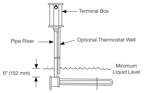
Over-the-Side Immersion Heater (bottom mount)
