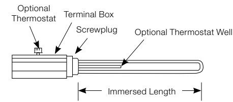
Screwplug Immersion Heater
