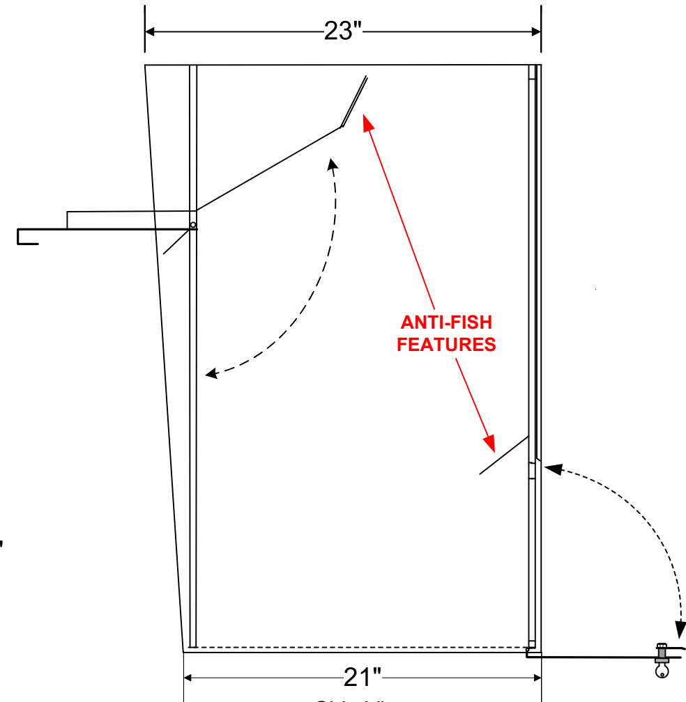
Side View
