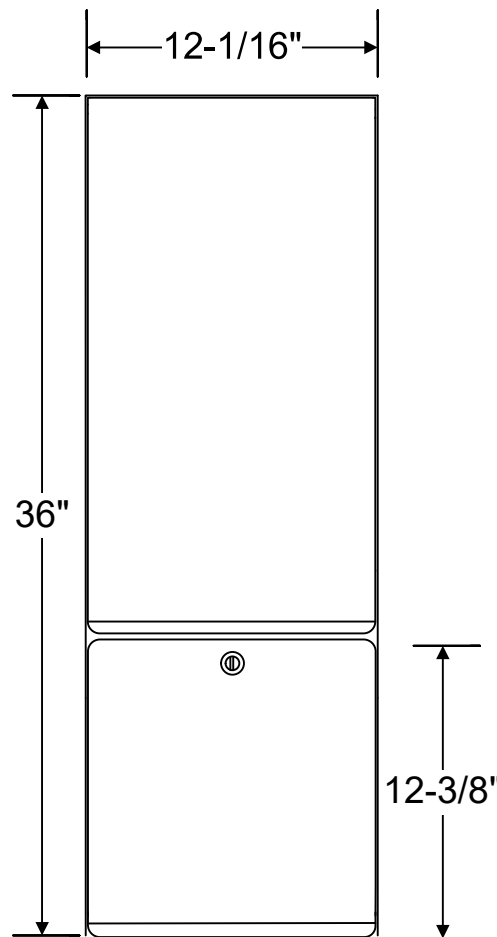
Rear View
