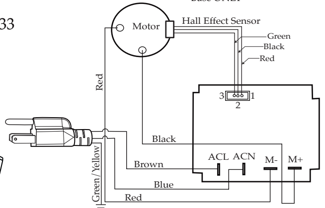
Wiring Diagram (on units after 11/1/2017)
